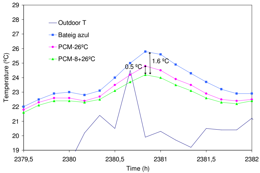
Figure 7. Temperature inside adiabatic boxes with one side of Bateig azul with and without PCMs. Effect of different melting temperature of PCMs during winter.
