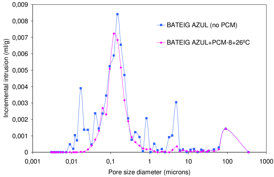
Figure 4. Mercury porosimetry for Bateig azul and Bateig azul treated with PCM-8+26°C.
